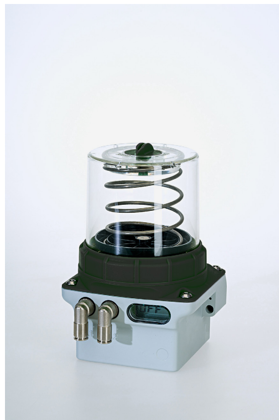
Figure 1: FP4 B212A front view
